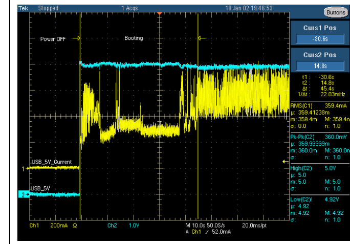
Fig 9: USB_5V Booting
